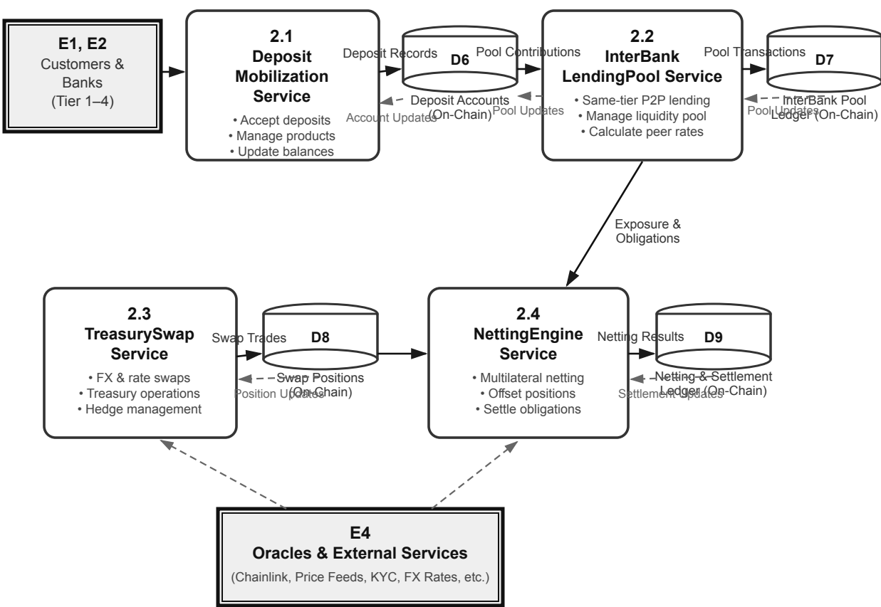
(C) Level-1 DFD – Treasury & Liquidity Subsystems
